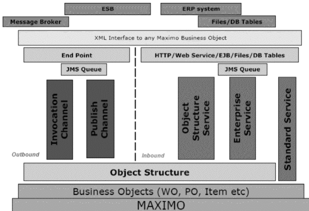
Figure 1. Tpae Integration Framework
